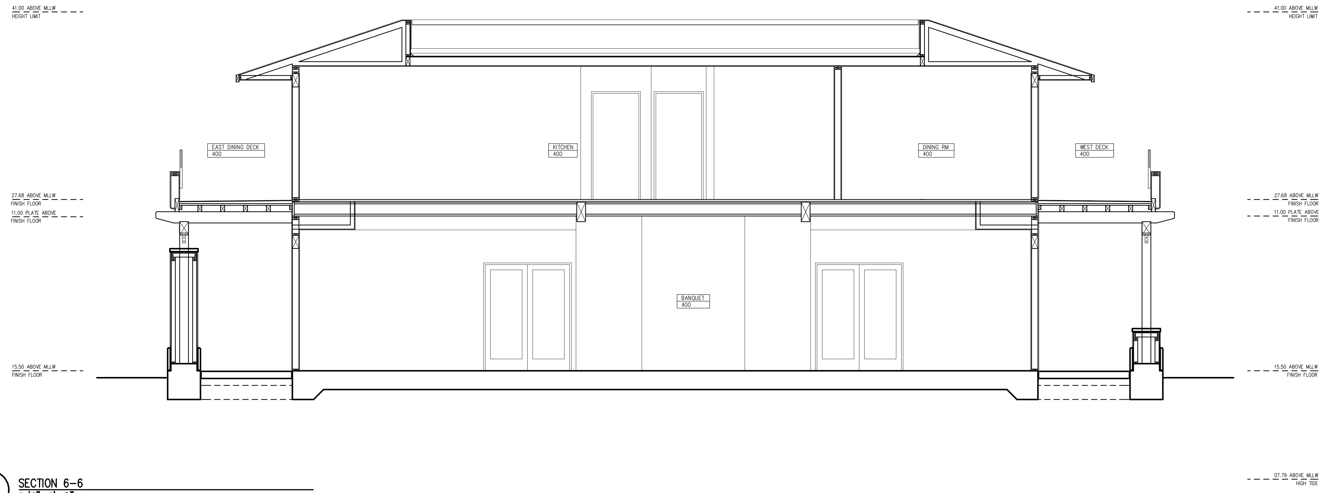
02 SECTION 6-6 1/4" = 1'-0"
